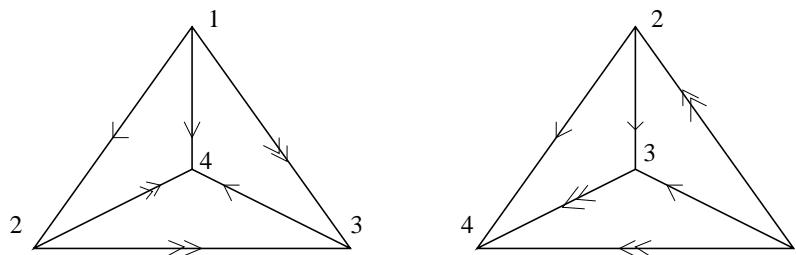
Figure 8: A quasi-simplicial ordered 3-cycle
